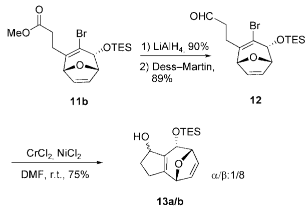
Scheme 3. Annulation by a Nozaki-Hiyama-Kishi closure.
