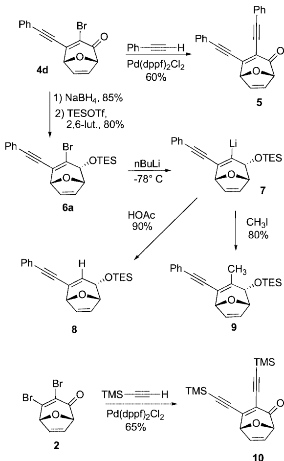
Scheme 2. Functionalization of the \alpha -bromide.
