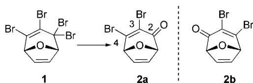
Scheme 1. Bicyclic building blocks containing a dibromoenone.
